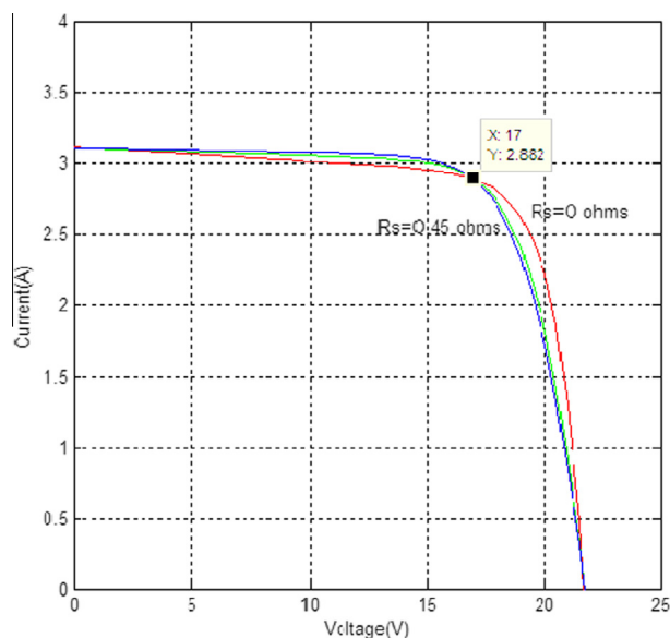
Fig. 15 I(V) characteristic for different R_S .
