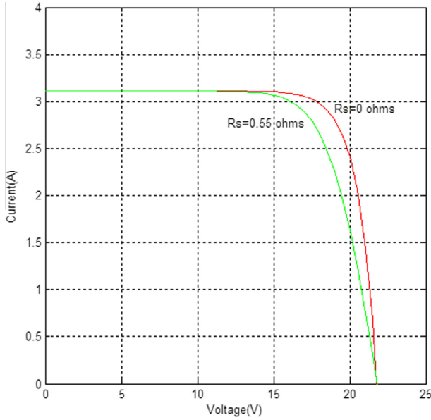
Fig. 10 I(V) characteristic in R_s model.
