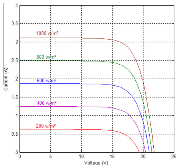
Fig. 16 I(V) characteristics by varying irradiance.
