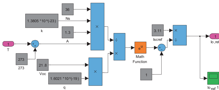
Fig. 4 Detailed I_{0,ref} implementation.
