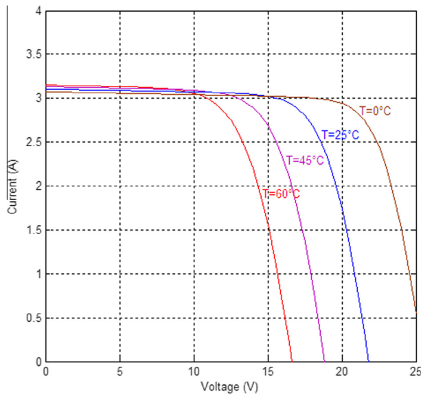
Fig. 17 I(V) characteristic by varying temperature.
