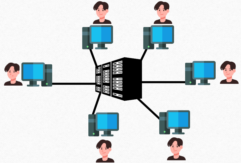
Figure 1.5 : Multi-User OS
