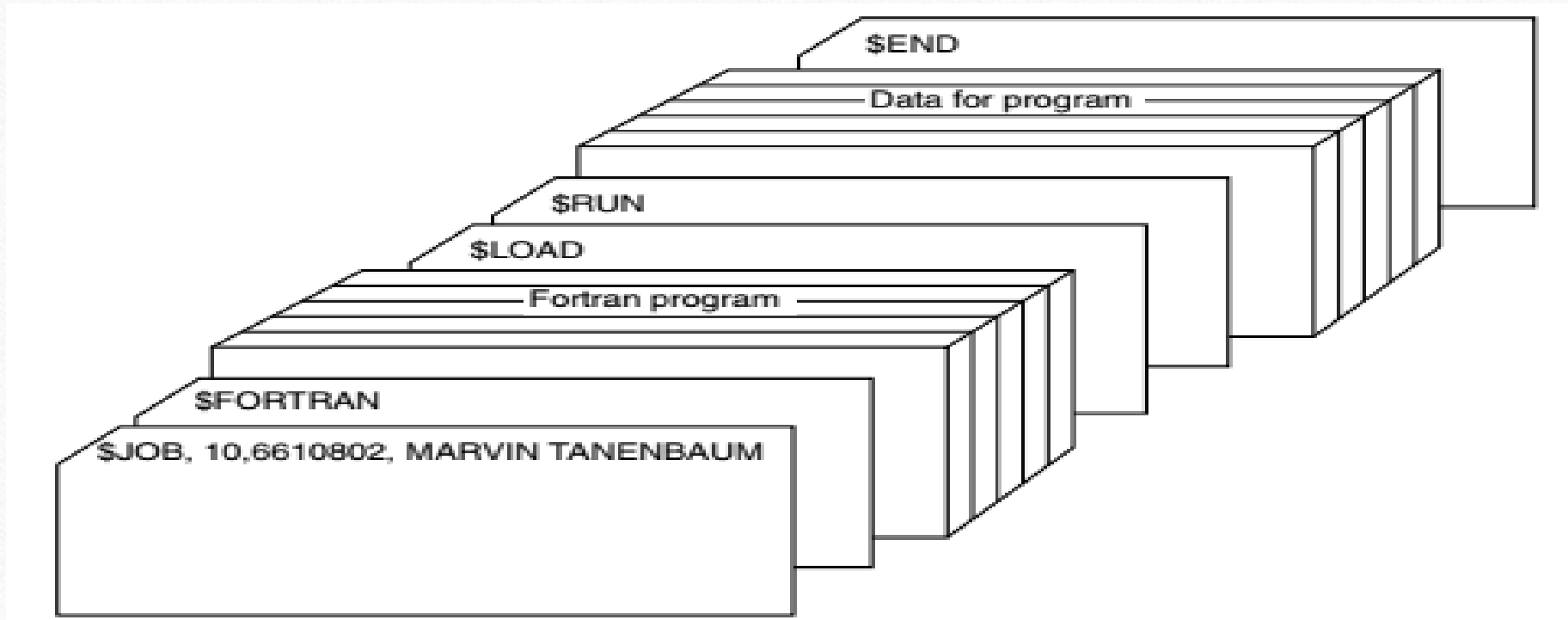
Figure 1.7 : Structure of a typical FMS job.
