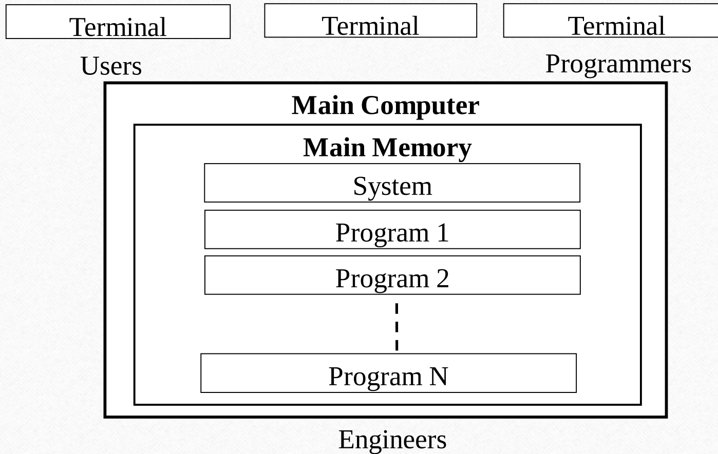
Figure 1.10 : A time-sharing system
