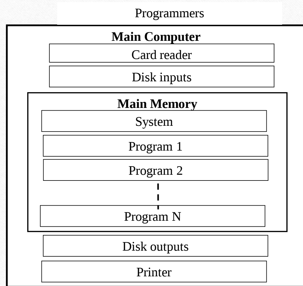
Figure 1.9 : A multiprogramming system
