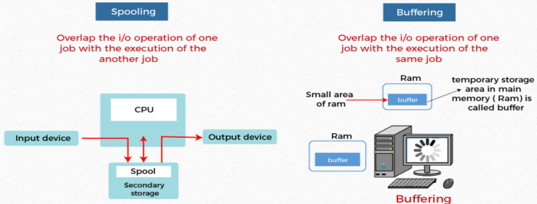
Figure 1.8 : Spooling and Buffering in OS
