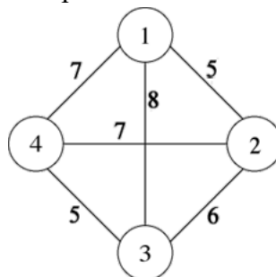
Figure III.6. Exemple de TSP.
